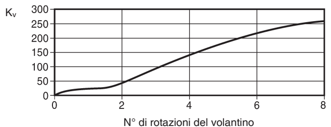
BSAT - DN200
