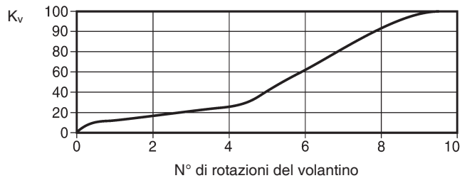
BSAT - DN125
